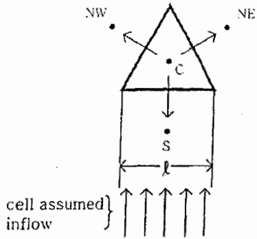
6a. Regular Square Cell
